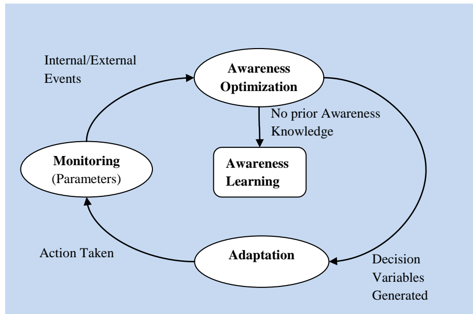
Figure 2.2 Optimization cycle
