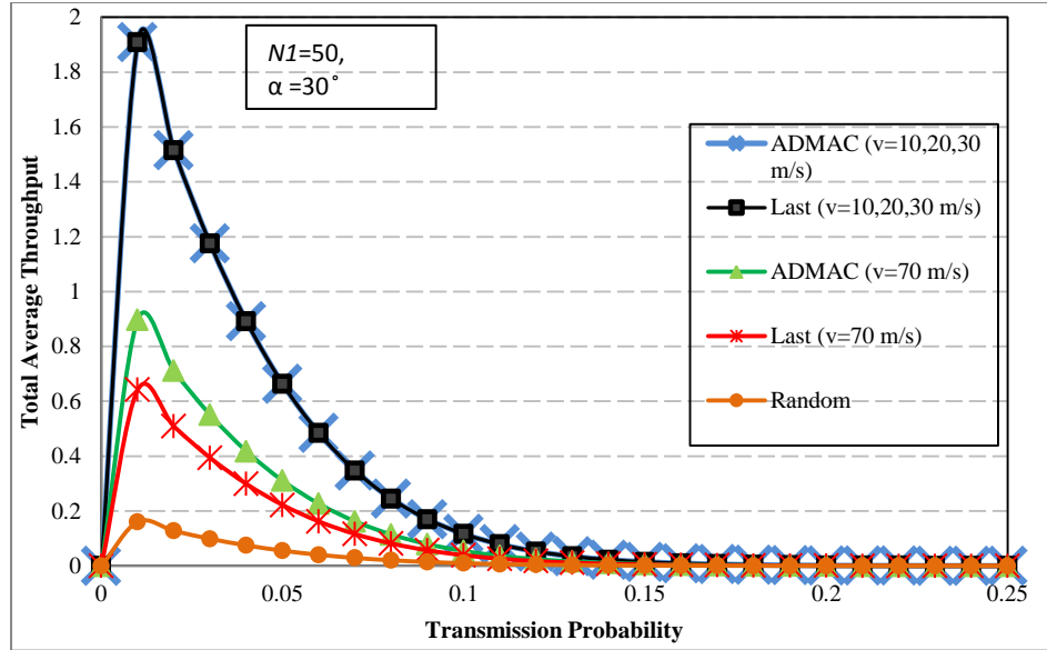
Figure 6.5 Total average throughput as a function of transmission probability for \alpha = 30^\circ and v = 10, 20, 30, 70 (m/s)
