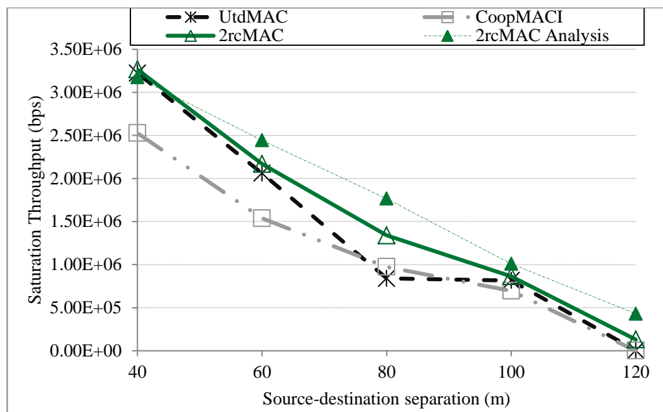
Figure 4.10: Saturation throughput comparison as a function of distance for 2rcMAC
